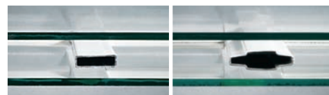
5/8" flat aluminum airspace grille
